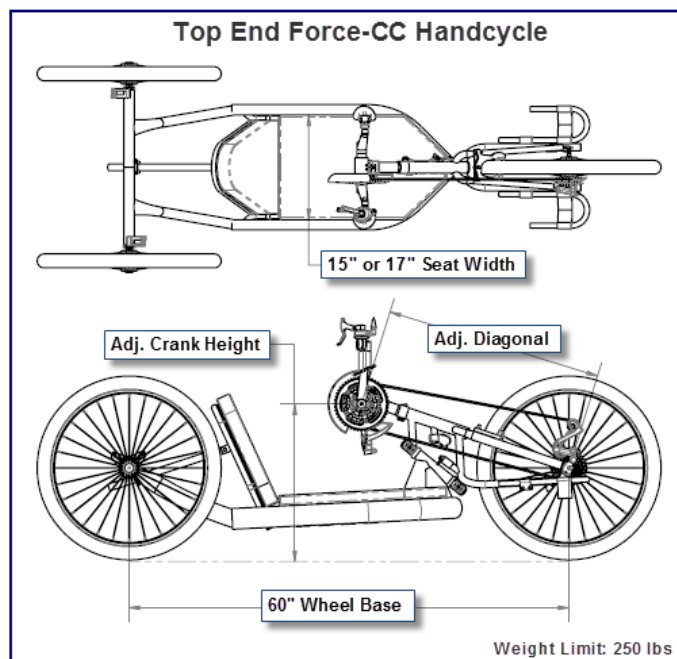
FORCE CC HANDCYCLE SPECIFICATIONS
